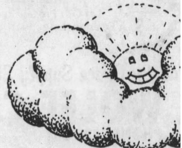
Clouds
